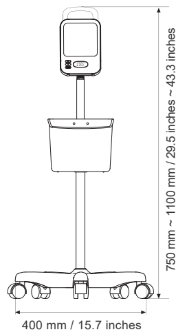
External Dimensions with optional stand
